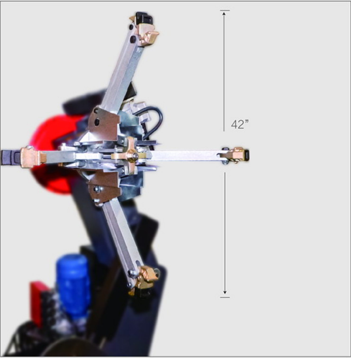
通用自动定心卡盘，操作尺寸从14" 到42" UNIVERSAL SELF-CENTRING CHUCK, OPERATE SIZE FROM 14" TO 42"
